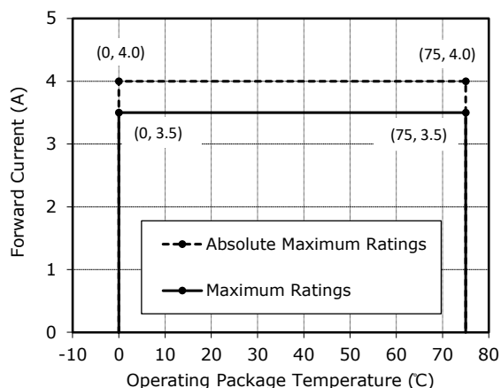
Figure 1. Derating Characteristics
