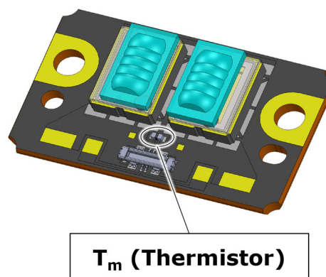
Figure 2. Temperature measurement point
