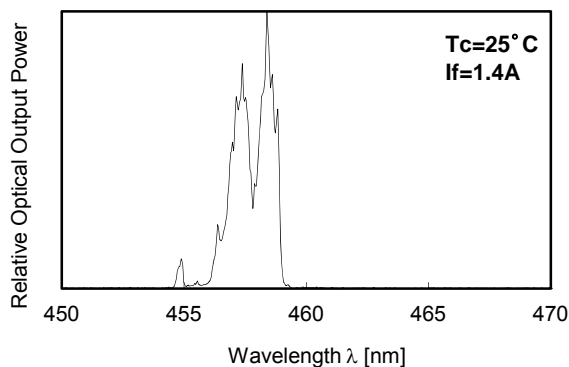
◆ Typical Spectrum
