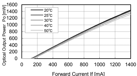
◆ Optical Output Power vs. Forward Current
